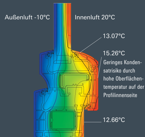
Corona CT 70 AS Cava Isothermen-Verlauf
